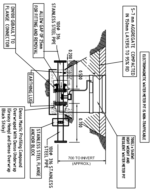
DETAIL OF DN100 FLOW METER INSTALLATION SCALE 1:25
