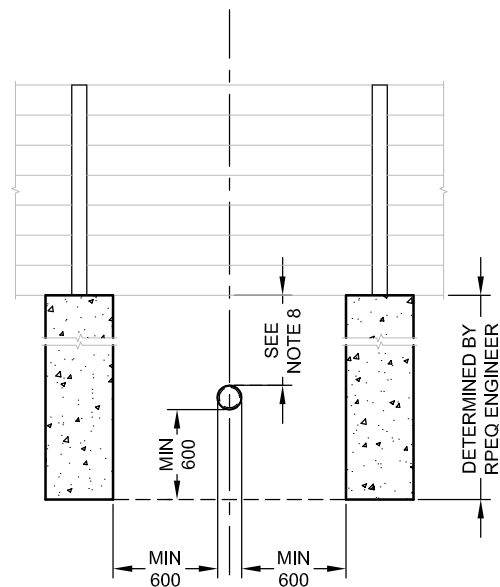
SECTION A
